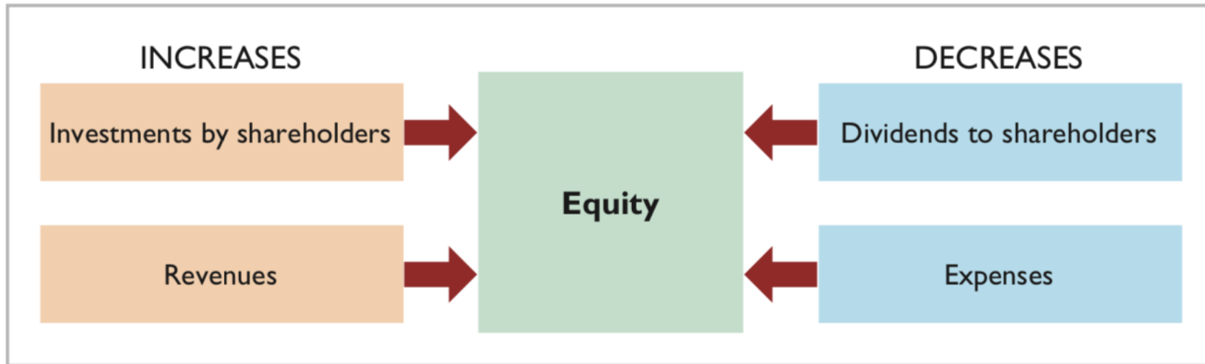
Illustration 1.7: Increases and decreases in equity.
